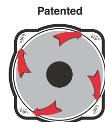
Patented Escape routes for impurities inside the rotor chamber
